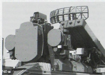
> The Osa-1T vehicle's day TV camera and thermal imager are mounted above the existing radar.
